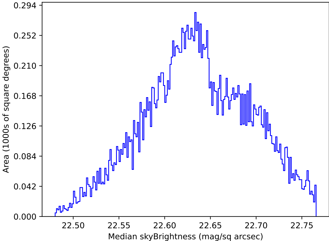
noroll_mjdp120_v3.4_10yrs Yr 1 u band: Median skyBrightness
