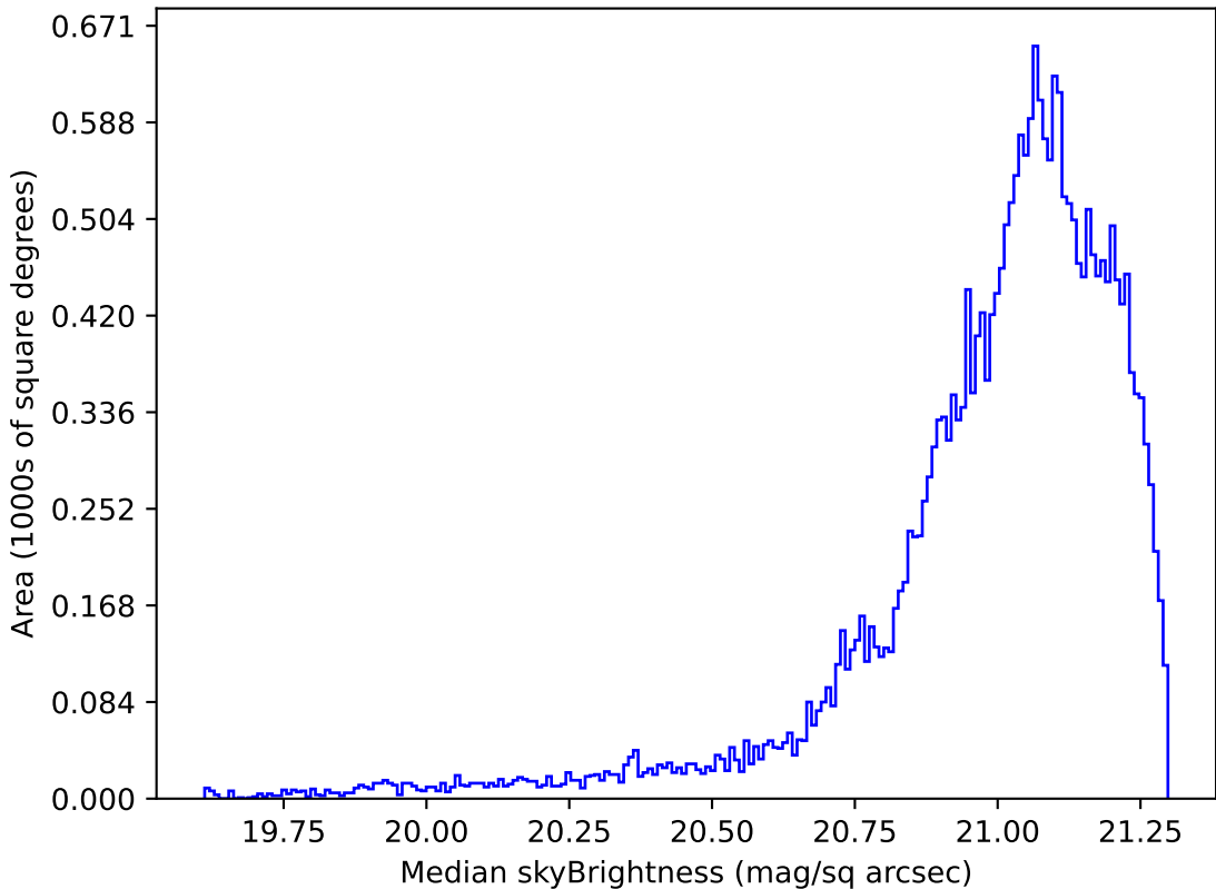
noroll_mjdp120_v3.4_10yrs Yr 1 r band: Median skyBrightness
