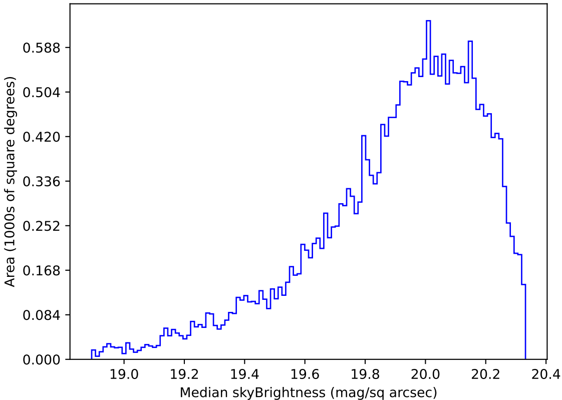
noroll_mjdp120_v3.4_10yrs Yr 1 i band: Median skyBrightness
