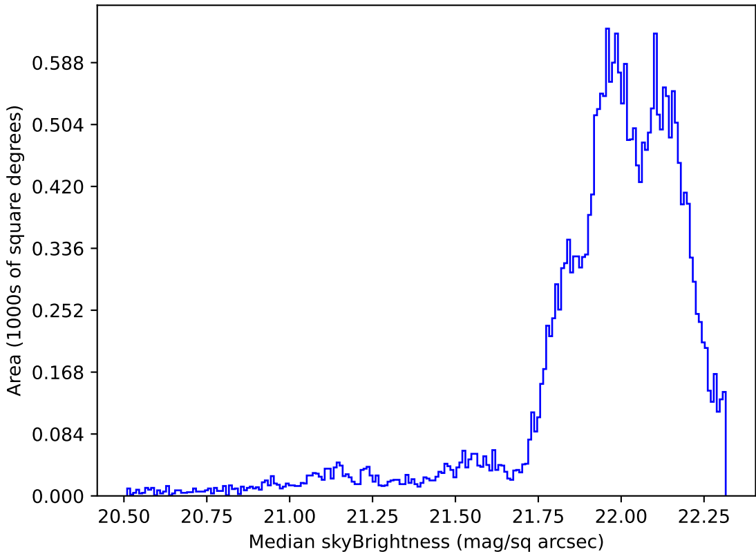
noroll_mjdp120_v3.4_10yrs Yr 1 g band: Median skyBrightness
