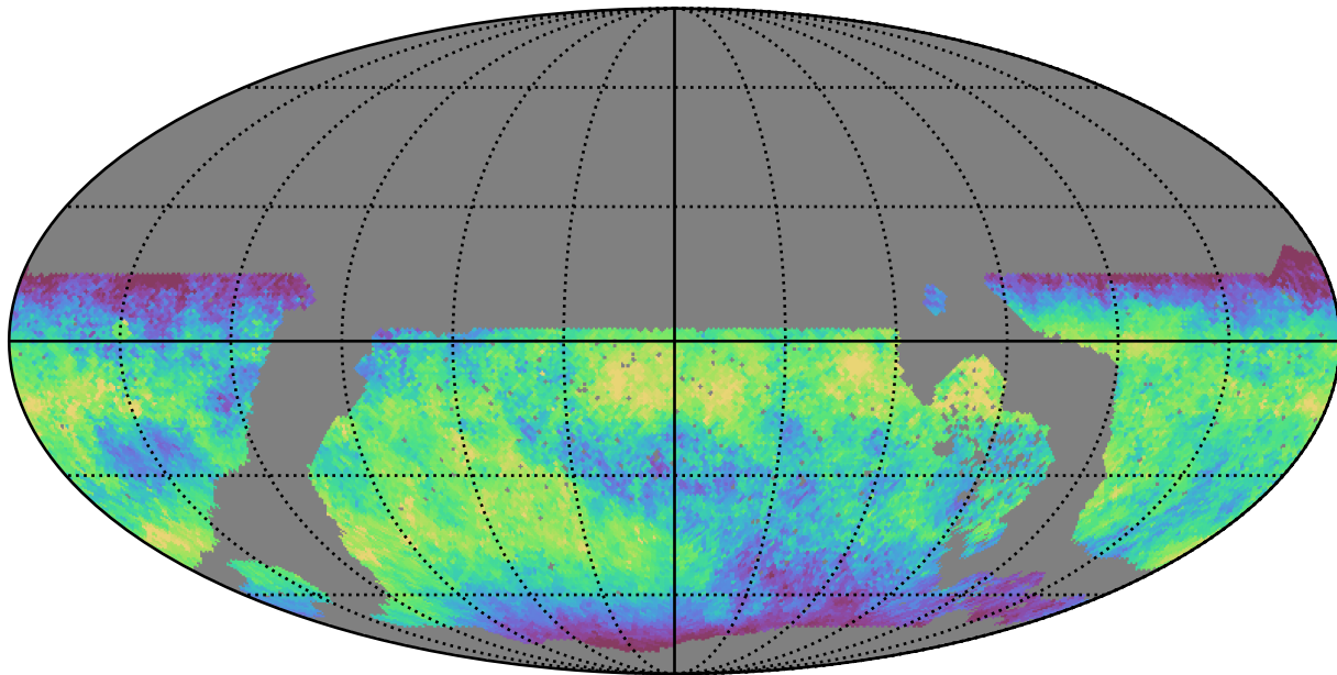
noroll_mjdp120_v3.4_10yrs WFD z band: Median skyBrightness
