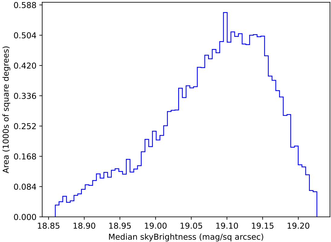
noroll_mjdp120_v3.4_10yrs WFD z band: Median skyBrightness
