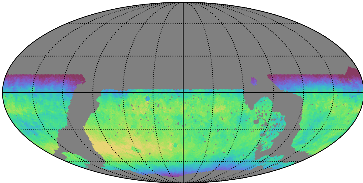
noroll_mjdp120_v3.4_10yrs WFD y band: Median skyBrightness
