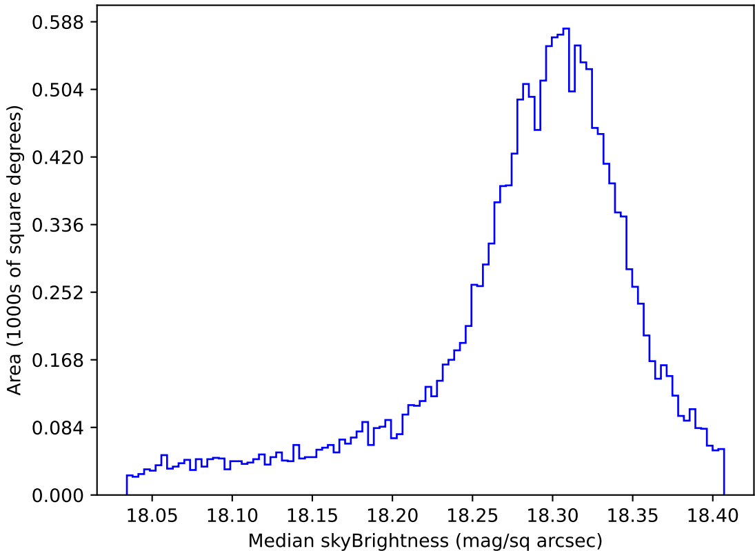
noroll_mjdp120_v3.4_10yrs WFD y band: Median skyBrightness
