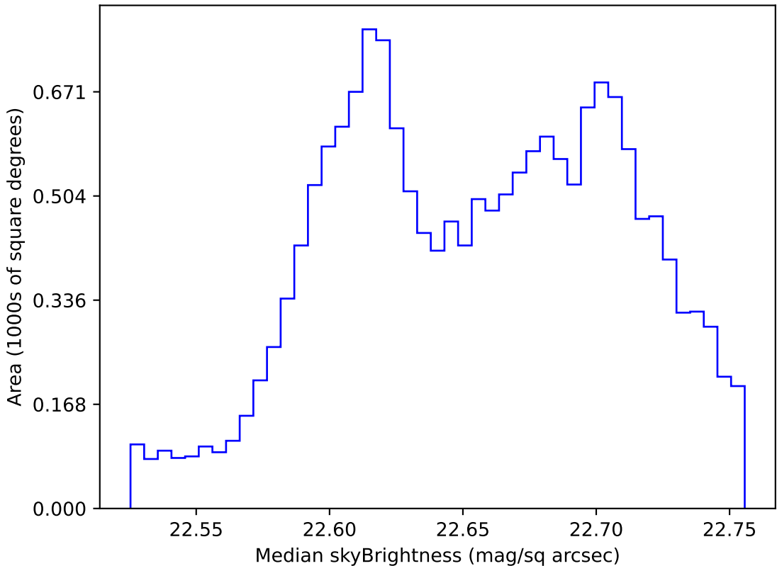
noroll_mjdp120_v3.4_10yrs WFD u band: Median skyBrightness
