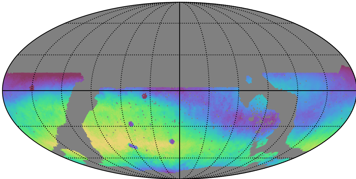
noroll_mjdp120_v3.4_10yrs WFD r band: Median skyBrightness
