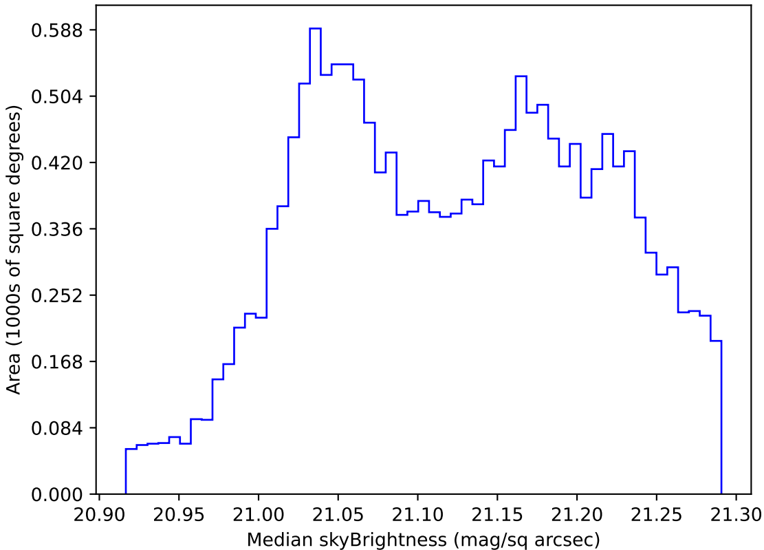
noroll_mjdp120_v3.4_10yrs WFD r band: Median skyBrightness
