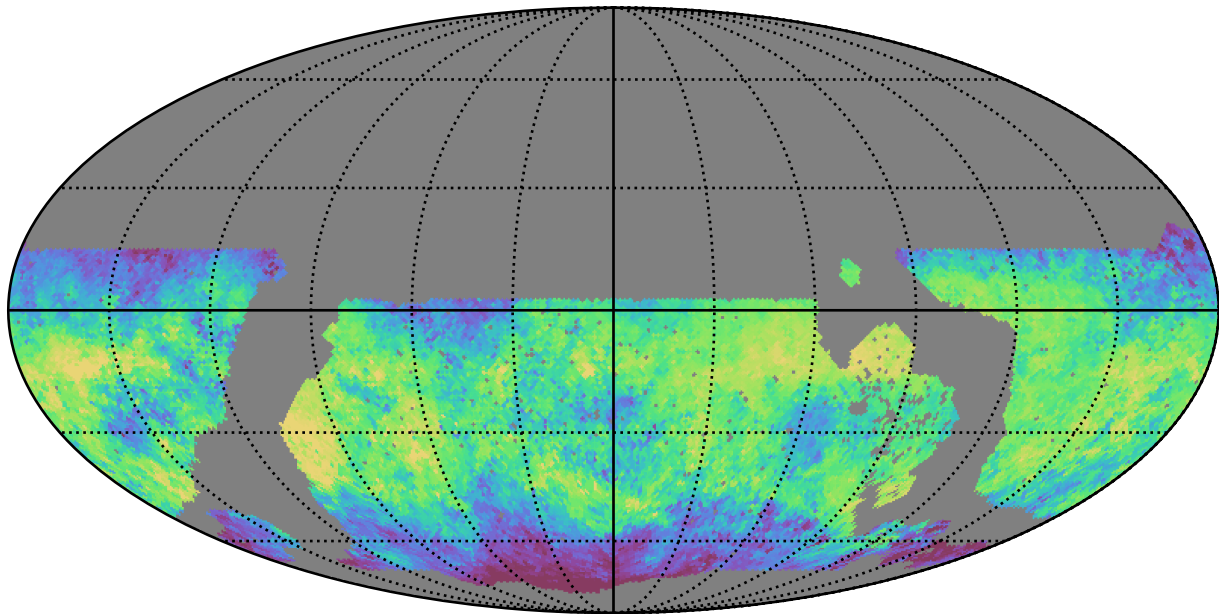
noroll_mjdp120_v3.4_10yrs WFD i band: Median skyBrightness
