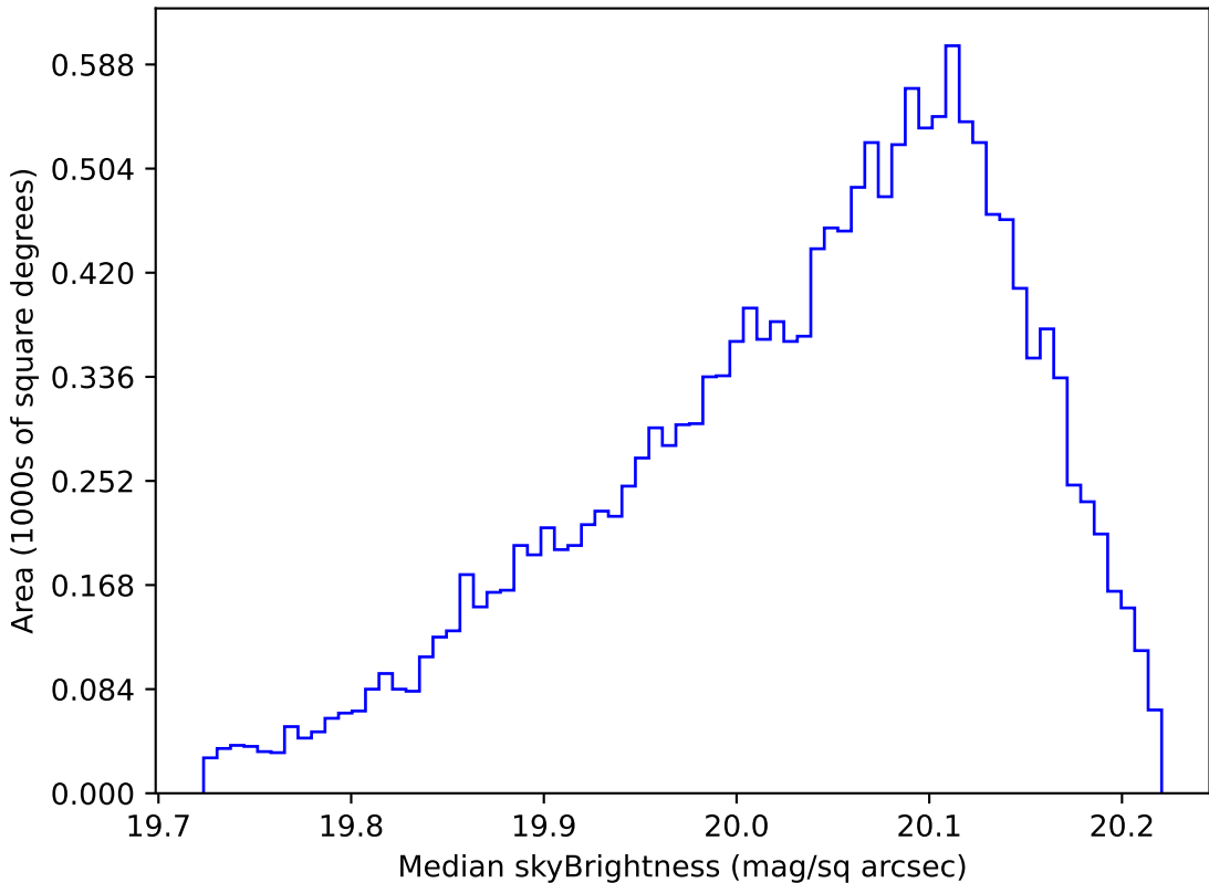
noroll_mjdp120_v3.4_10yrs WFD i band: Median skyBrightness
