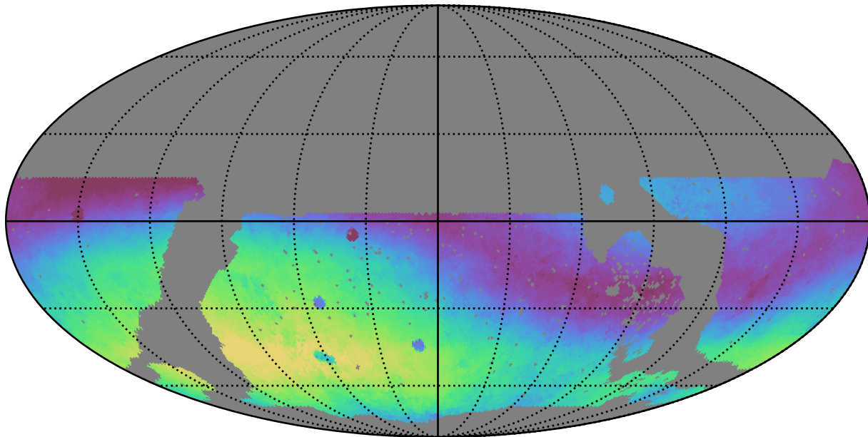
noroll_mjdp120_v3.4_10yrs WFD g band: Median skyBrightness
