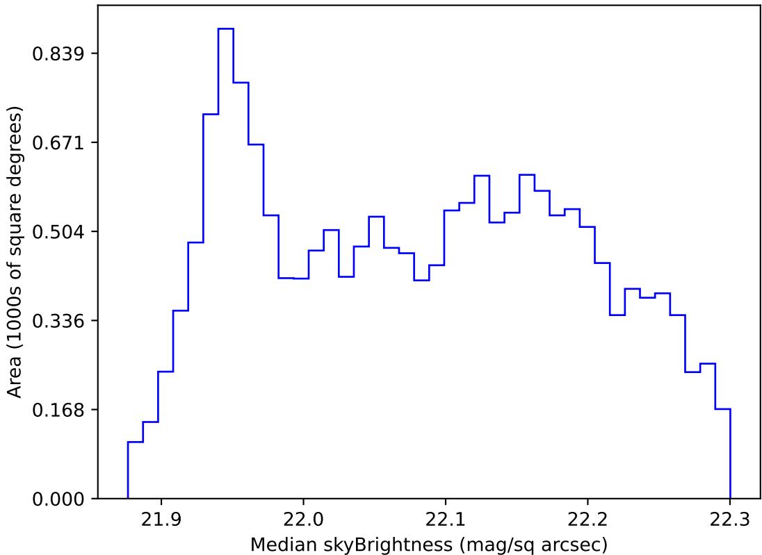
noroll_mjdp120_v3.4_10yrs WFD g band: Median skyBrightness
