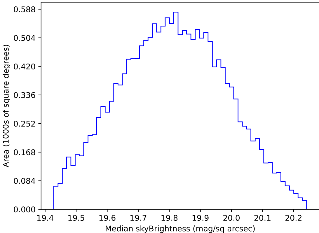
noroll_mjdp120_v3.4_10yrs WFD all bands: Median skyBrightness
