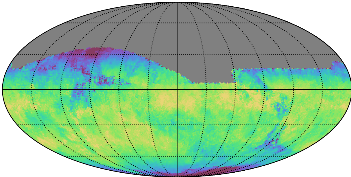
noroll_mjdp120_v3.4_10yrs All sky z band: Median skyBrightness
