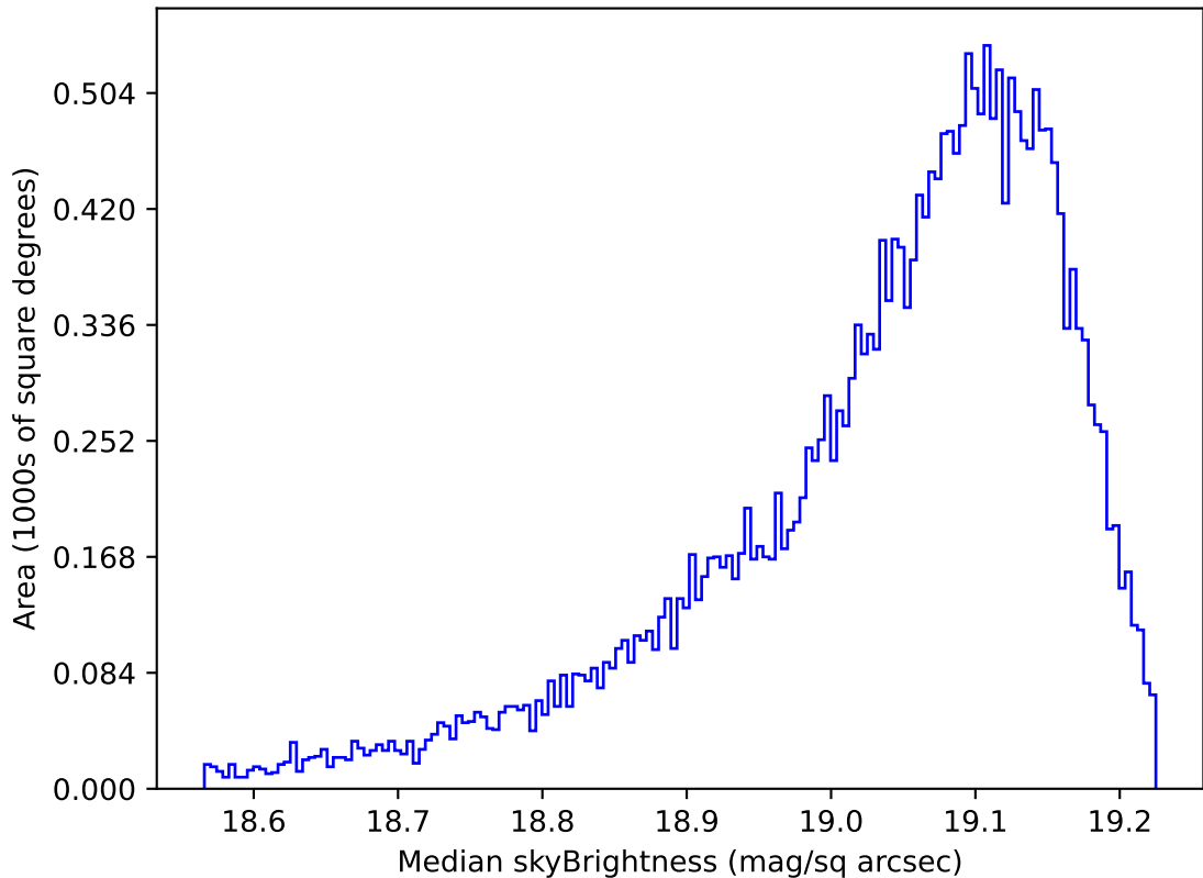
noroll_mjdp120_v3.4_10yrs All sky z band: Median skyBrightness
