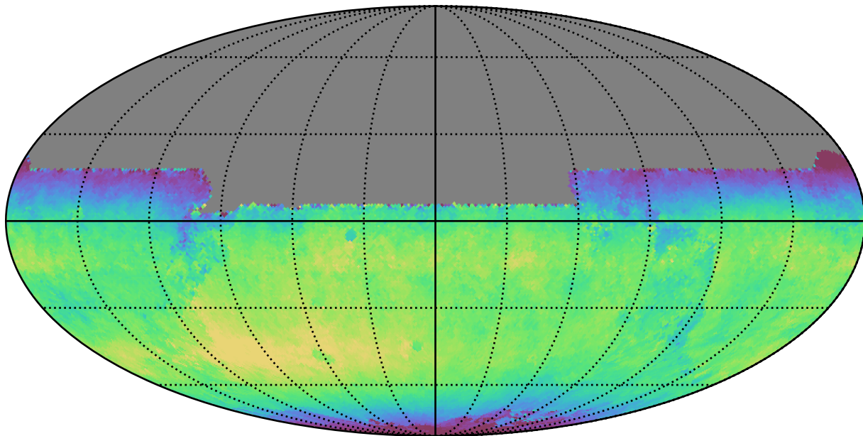
noroll_mjdp120_v3.4_10yrs All sky y band: Median skyBrightness
