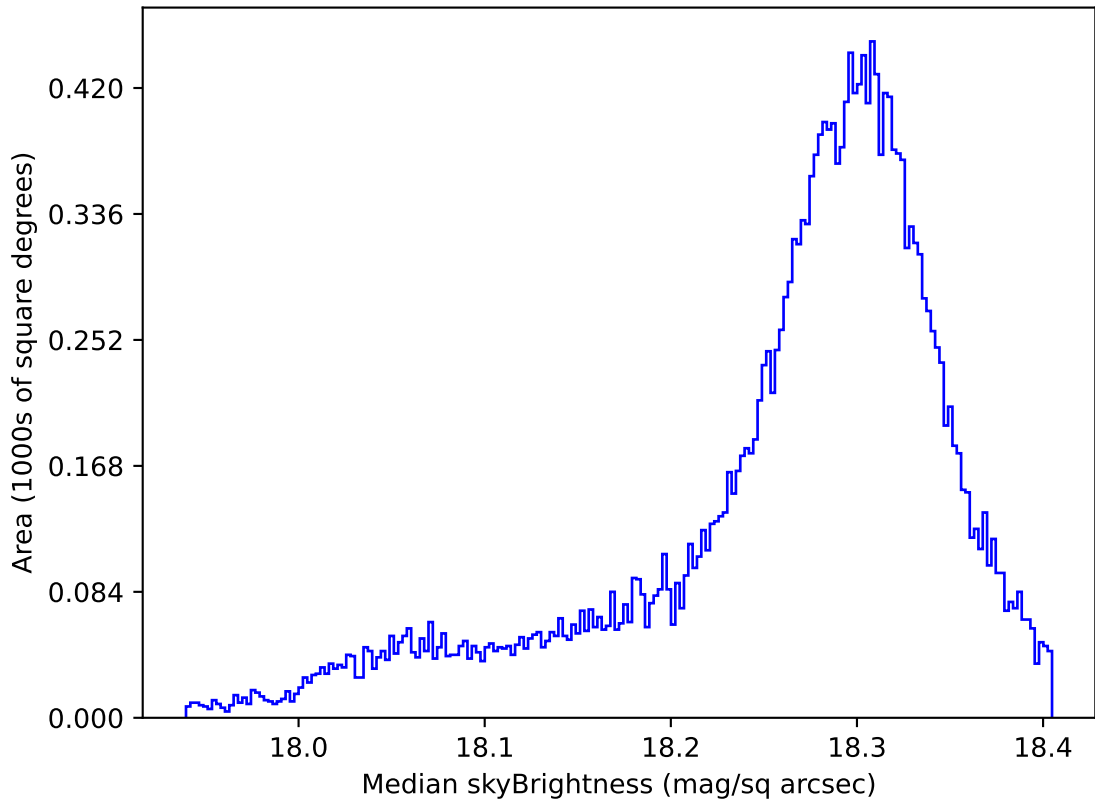
noroll_mjdp120_v3.4_10yrs All sky y band: Median skyBrightness
