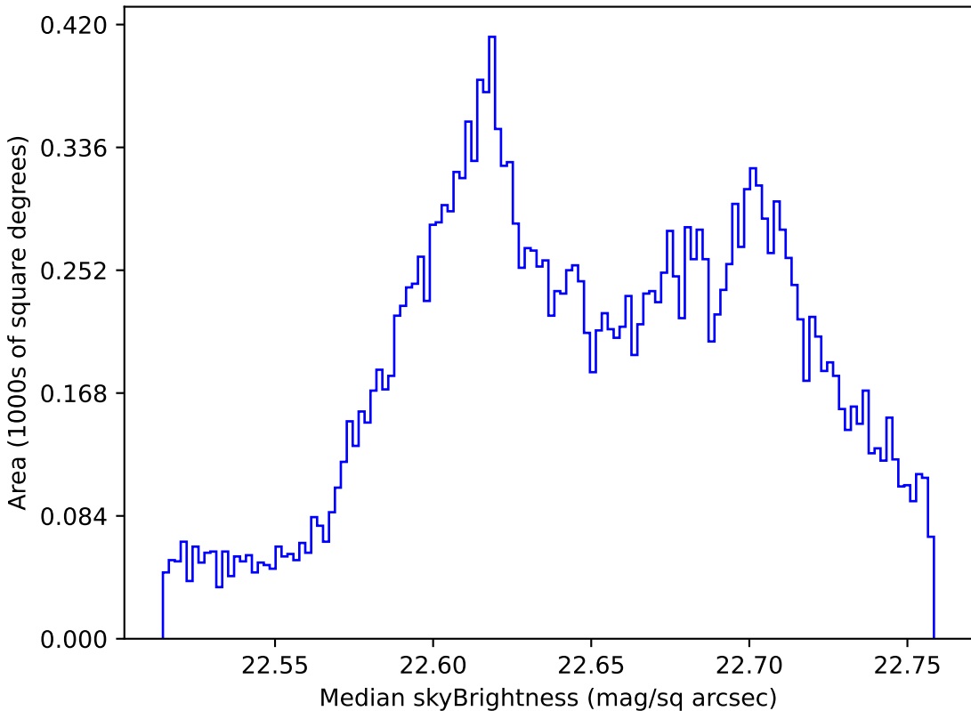
noroll_mjdp120_v3.4_10yrs All sky u band: Median skyBrightness
