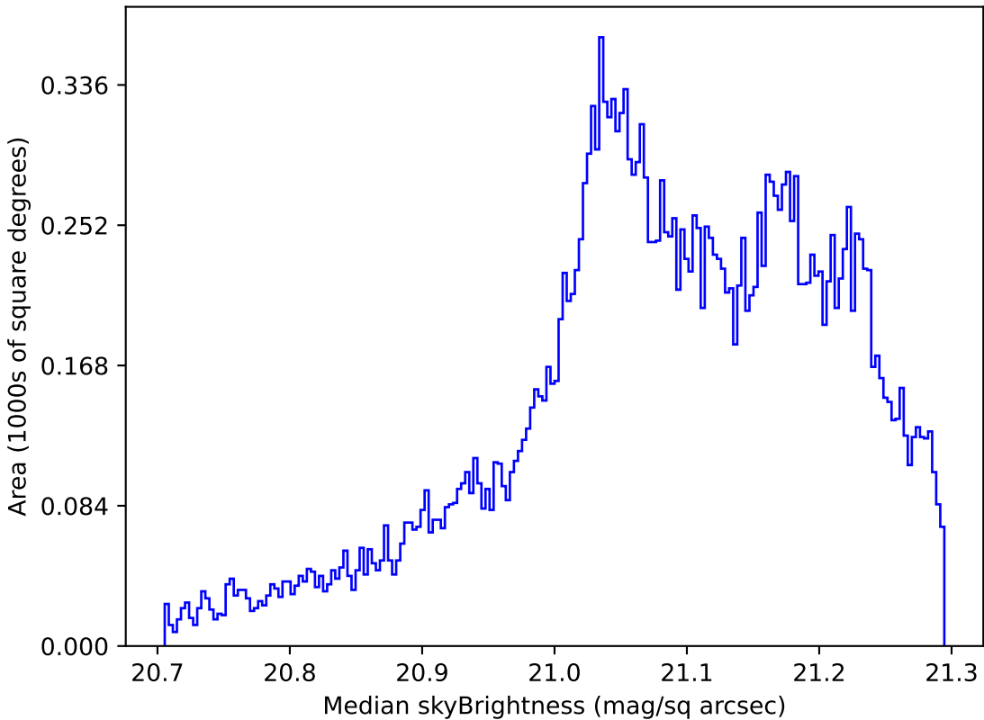
noroll_mjdp120_v3.4_10yrs All sky r band: Median skyBrightness
