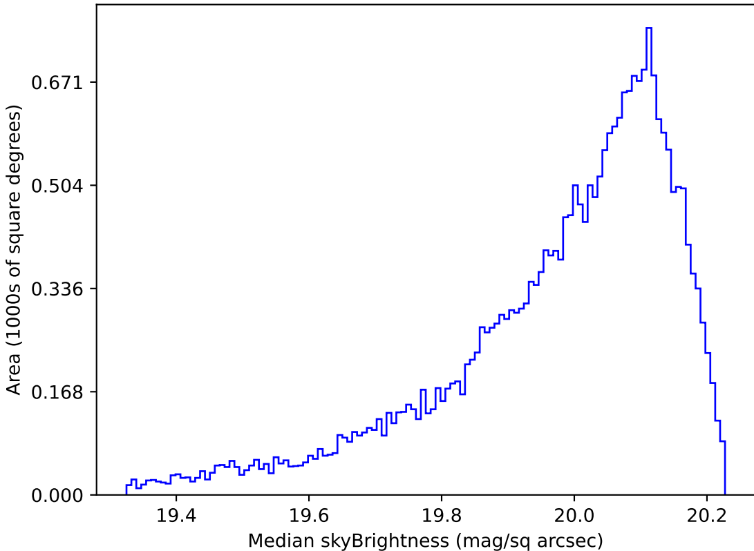
noroll_mjdp120_v3.4_10yrs All sky i band: Median skyBrightness
