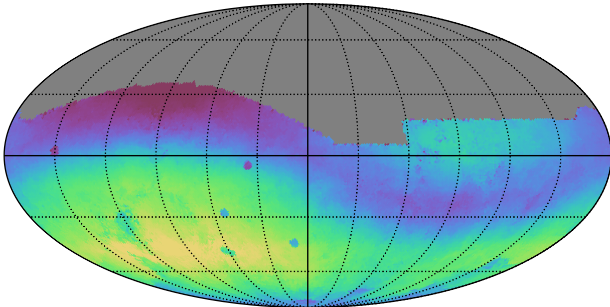
noroll_mjdp120_v3.4_10yrs All sky g band: Median skyBrightness
