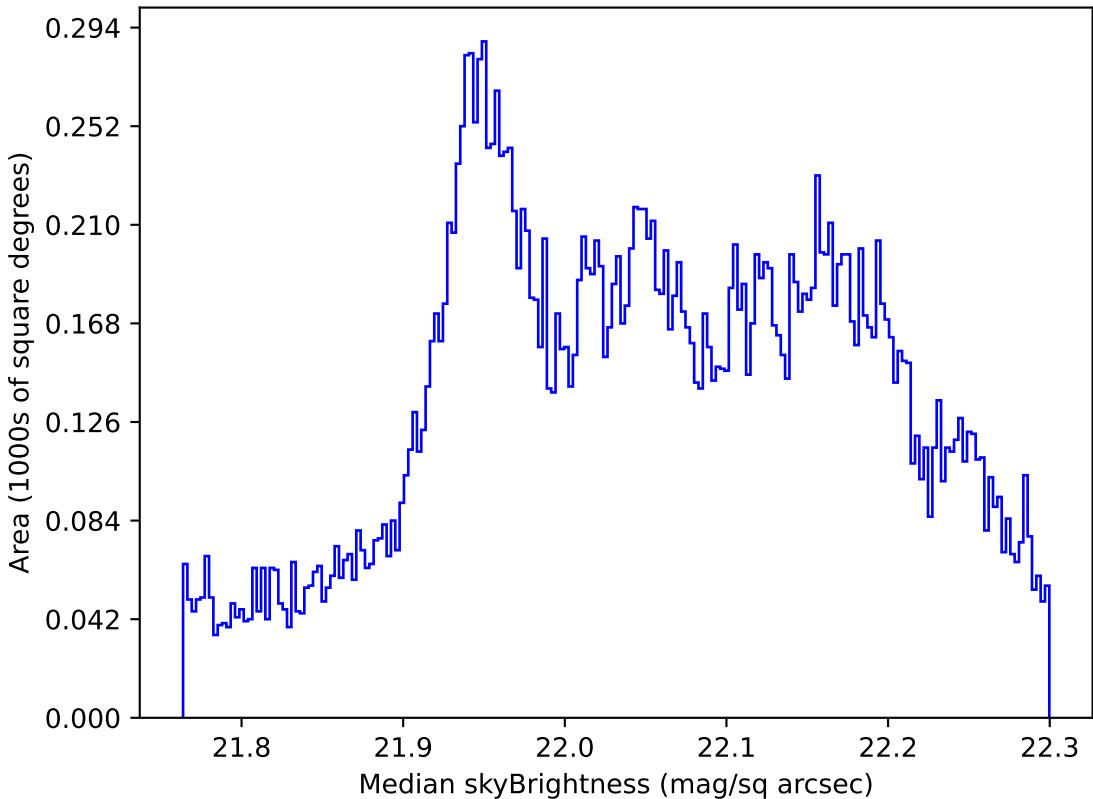
noroll_mjdp120_v3.4_10yrs All sky g band: Median skyBrightness
