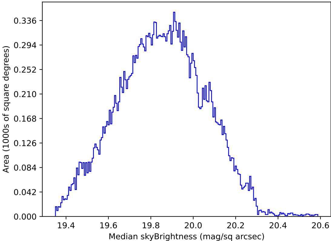
noroll_mjdp120_v3.4_10yrs All sky all bands: Median skyBrightness
