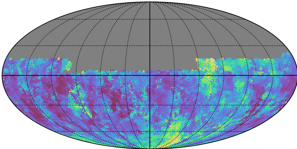
noroll_mjdp120_v3.4_10yrs Yr 1 u band: Median seeingGeom
