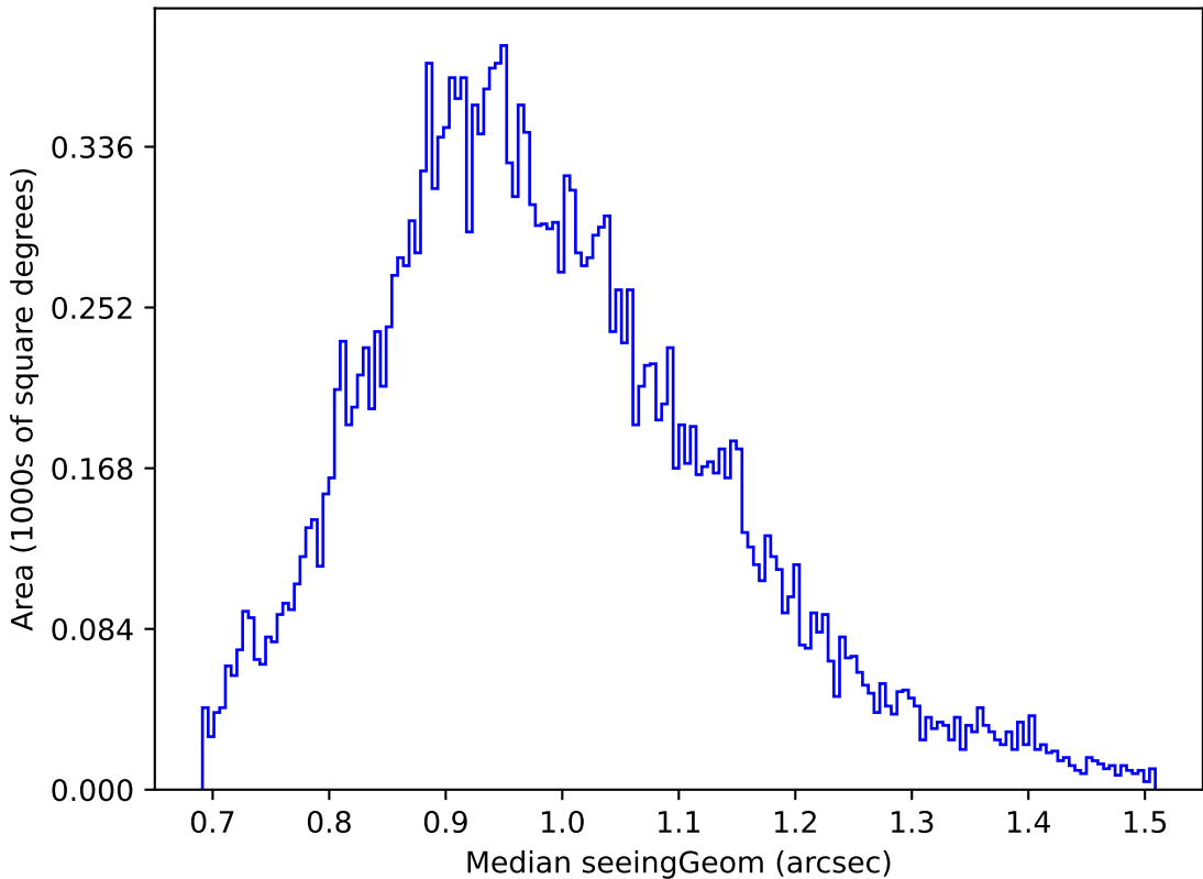
noroll_mjdp120_v3.4_10yrs Yr 1 u band: Median seeingGeom
