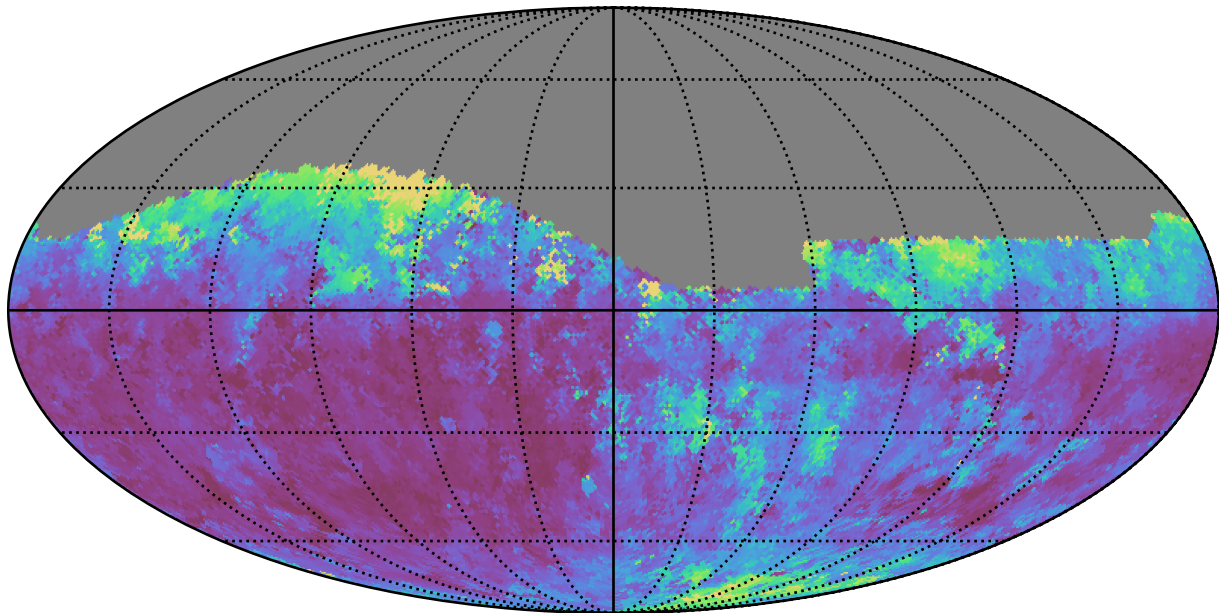
noroll_mjdp120_v3.4_10yrs Yr 1 i band: Median seeingGeom
