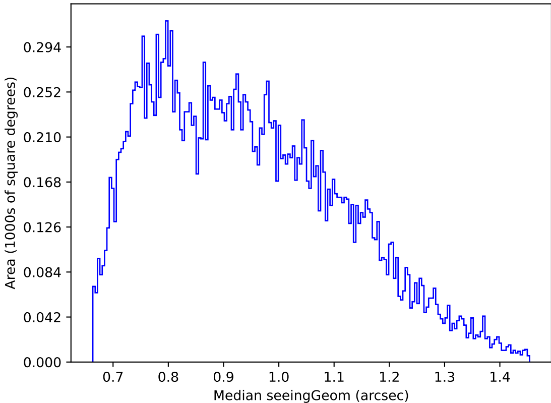
noroll_mjdp120_v3.4_10yrs Yr 1 g band: Median seeingGeom
