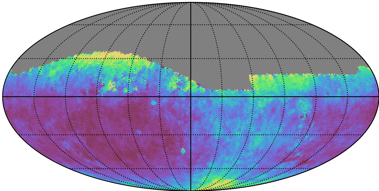
noroll_mjdp120_v3.4_10yrs Yr 1 all bands: Median seeingGeom
