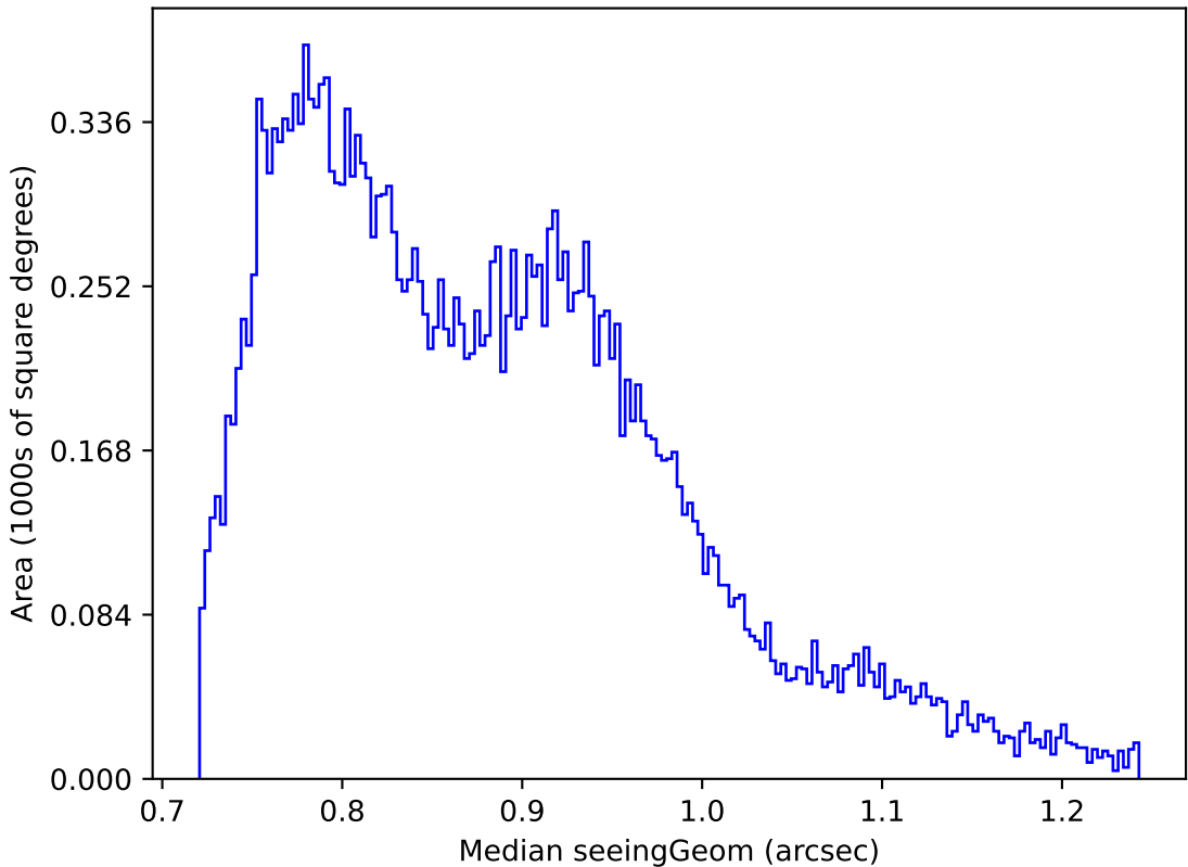
noroll_mjdp120_v3.4_10yrs Yr 1 all bands: Median seeingGeom
