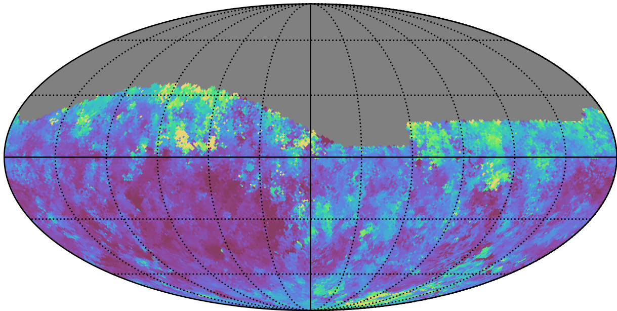
noroll_mjdp120_v3.4_10yrs Yr 1 z band: Median seeingEff
