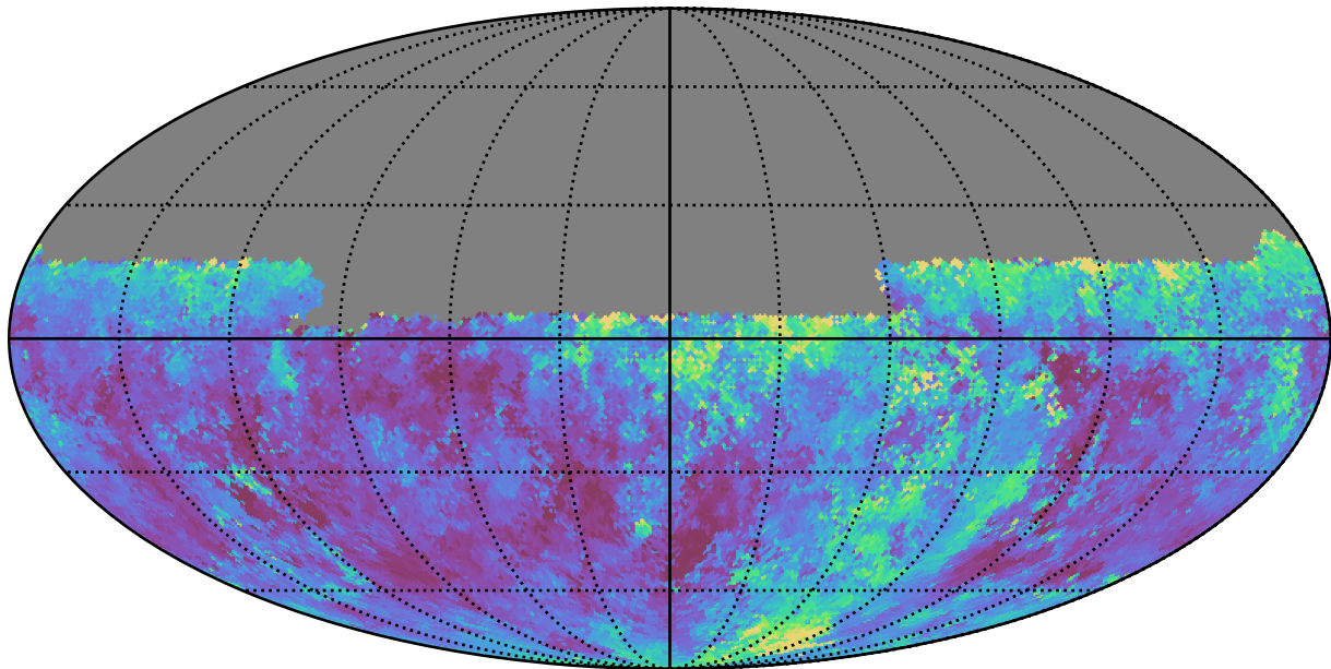
noroll_mjdp120_v3.4_10yrs Yr 1 y band: Median seeingEff
