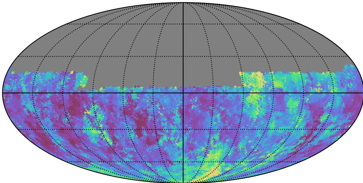
noroll_mjdp120_v3.4_10yrs Yr 1 u band: Median seeingEff
