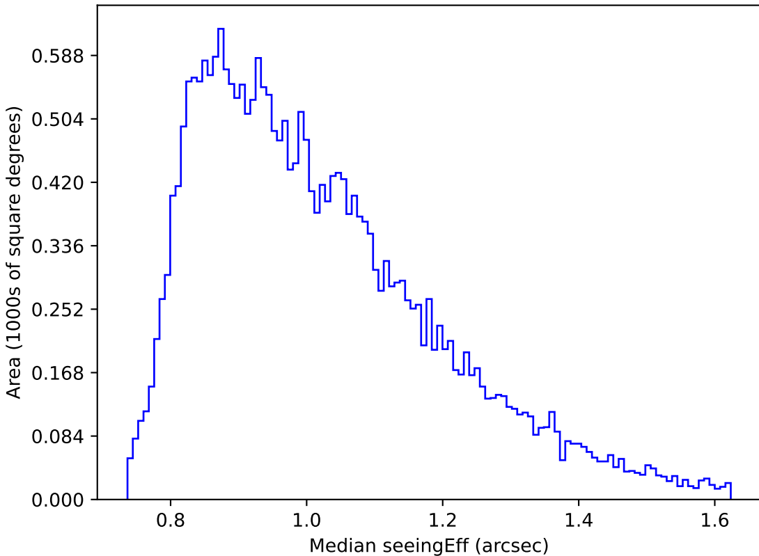
noroll_mjdp120_v3.4_10yrs Yr 1 r band: Median seeingEff
