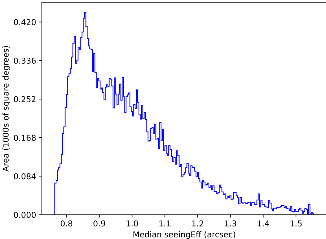
noroll_mjdp120_v3.4_10yrs Yr 1 i band: Median seeingEff
