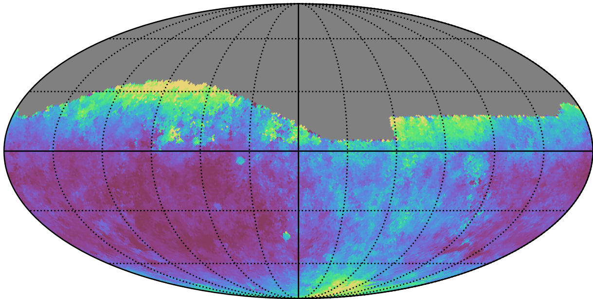
noroll_mjdp120_v3.4_10yrs Yr 1 all bands: Median seeingEff
