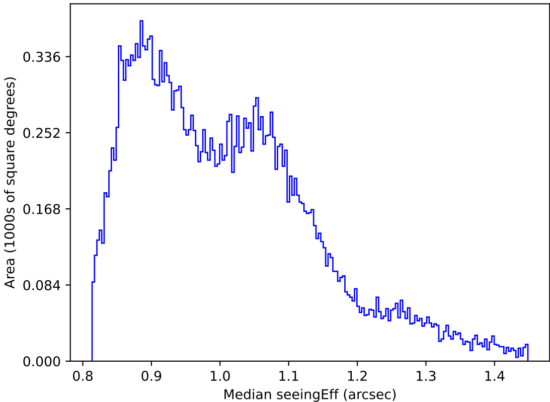
noroll_mjdp120_v3.4_10yrs Yr 1 all bands: Median seeingEff
