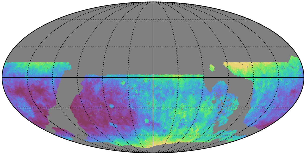
noroll_mjdp120_v3.4_10yrs WFD z band: Median seeingEff
