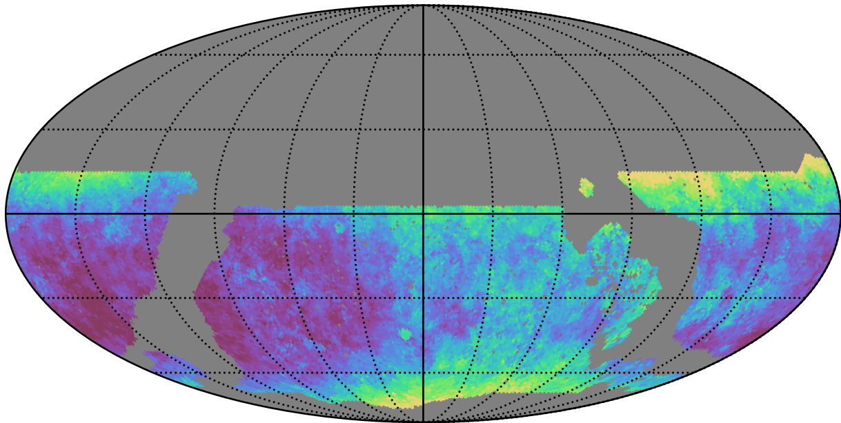
noroll_mjdp120_v3.4_10yrs WFD y band: Median seeingEff
