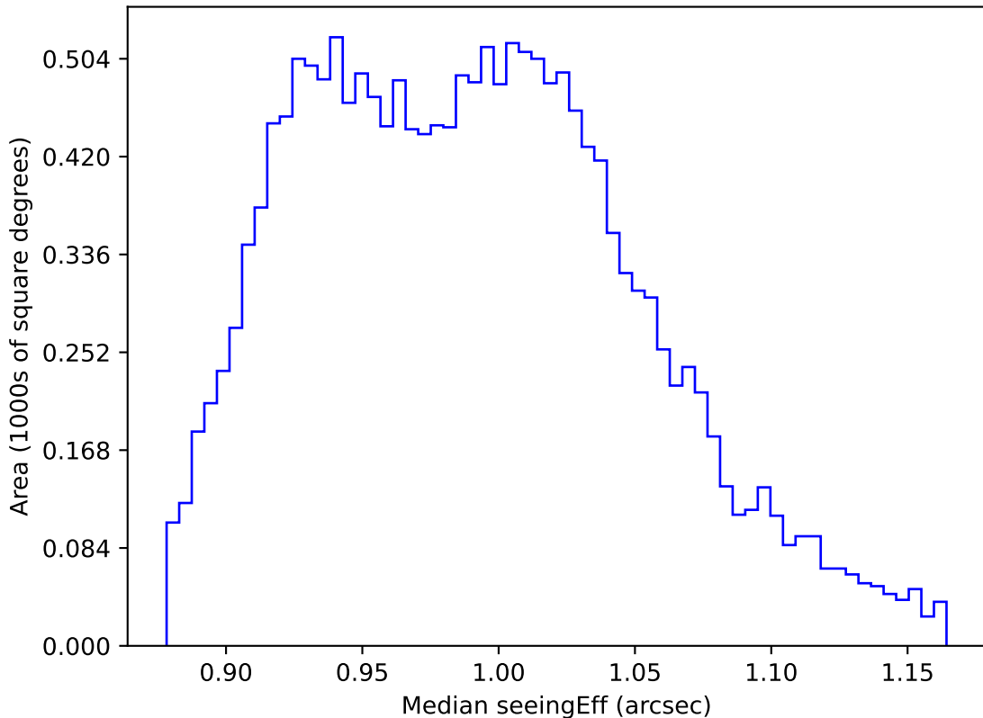
noroll_mjdp120_v3.4_10yrs WFD y band: Median seeingEff
