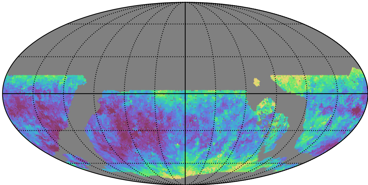
noroll_mjdp120_v3.4_10yrs WFD u band: Median seeingEff
