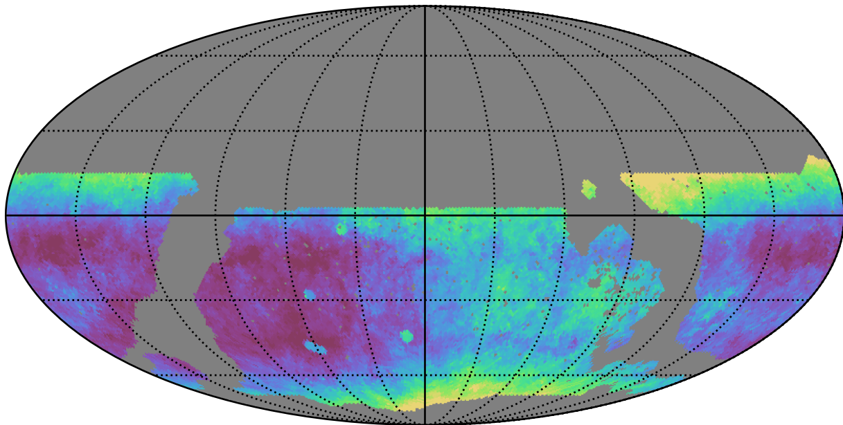
noroll_mjdp120_v3.4_10yrs WFD r band: Median seeingEff
