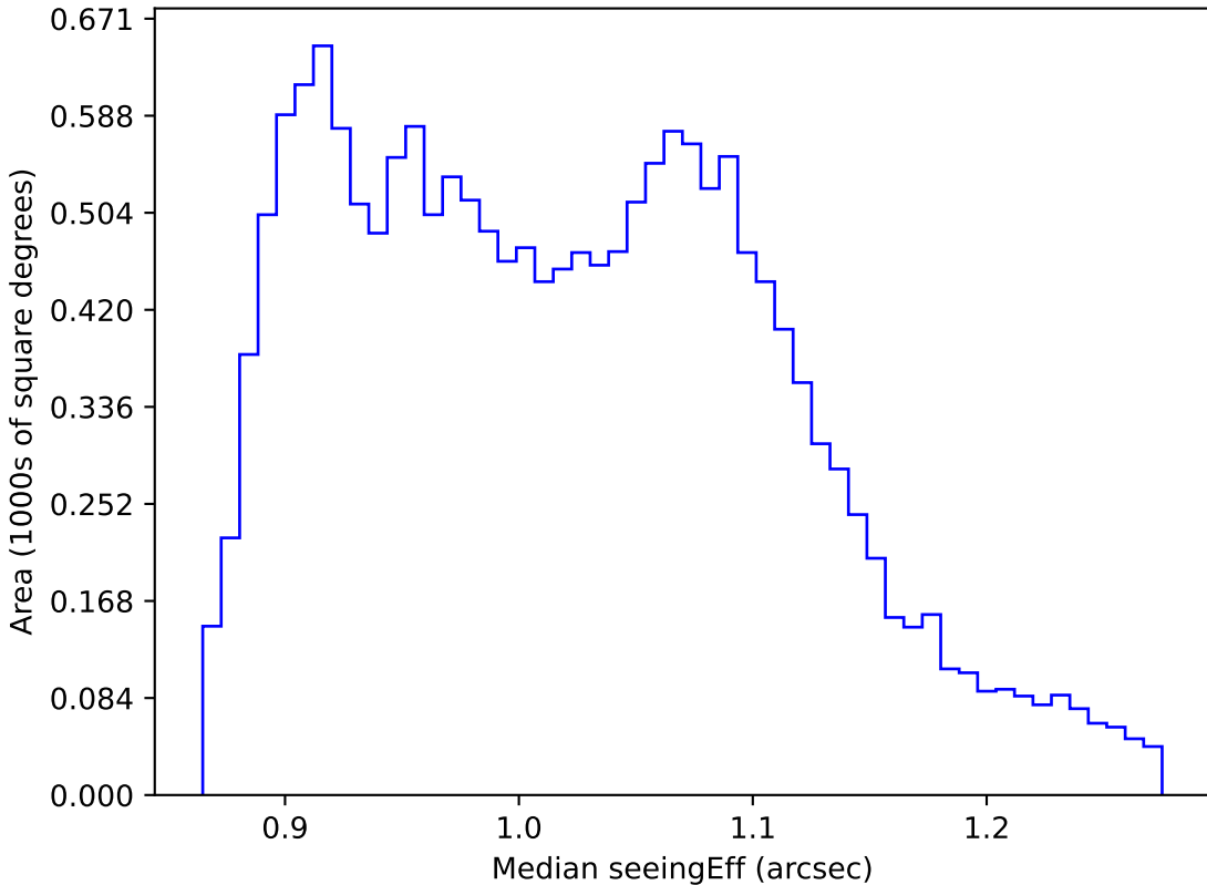
noroll_mjdp120_v3.4_10yrs WFD r band: Median seeingEff
