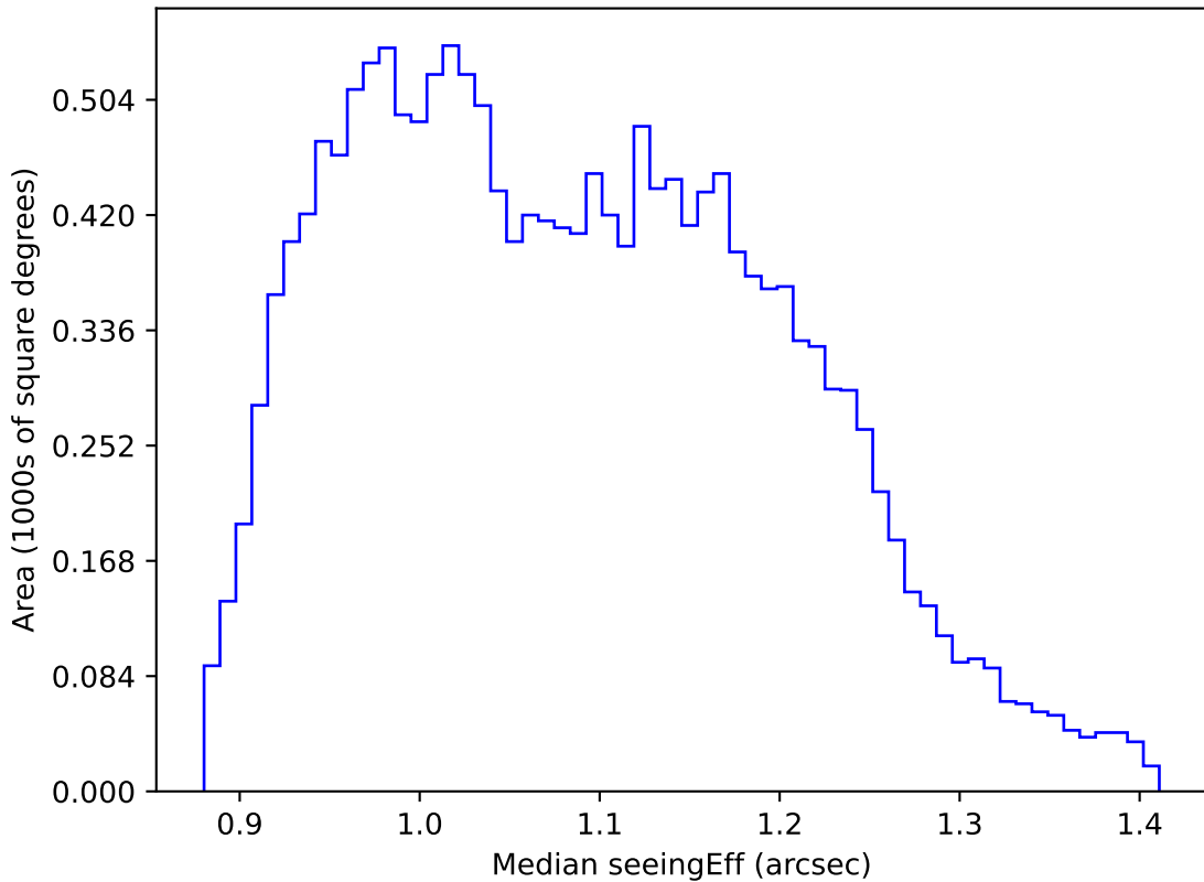
noroll_mjdp120_v3.4_10yrs WFD g band: Median seeingEff
