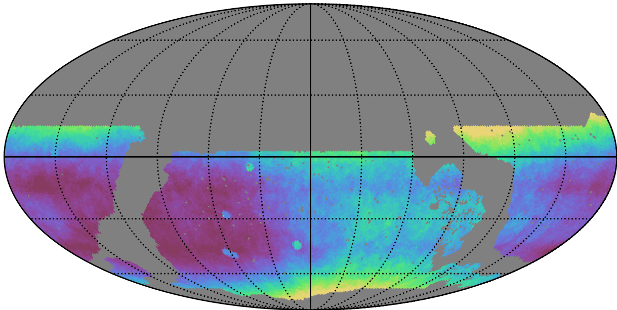
noroll_mjdp120_v3.4_10yrs WFD all bands: Median seeingEff
