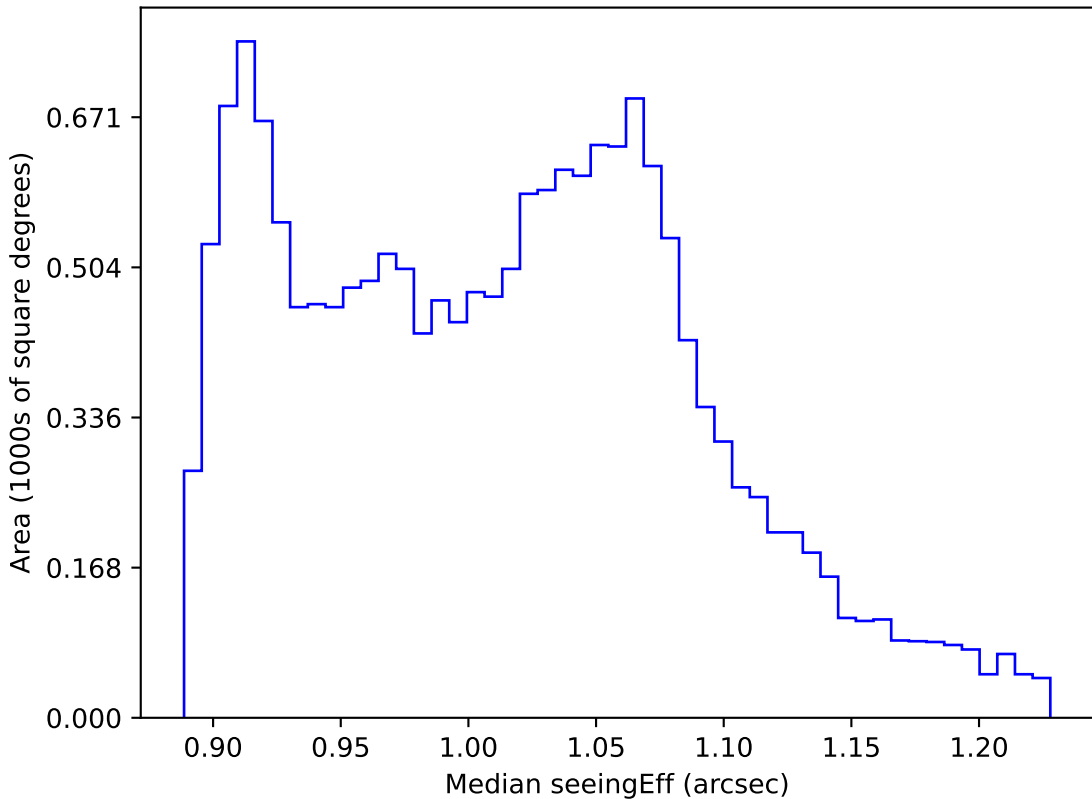
noroll_mjdp120_v3.4_10yrs WFD all bands: Median seeingEff
