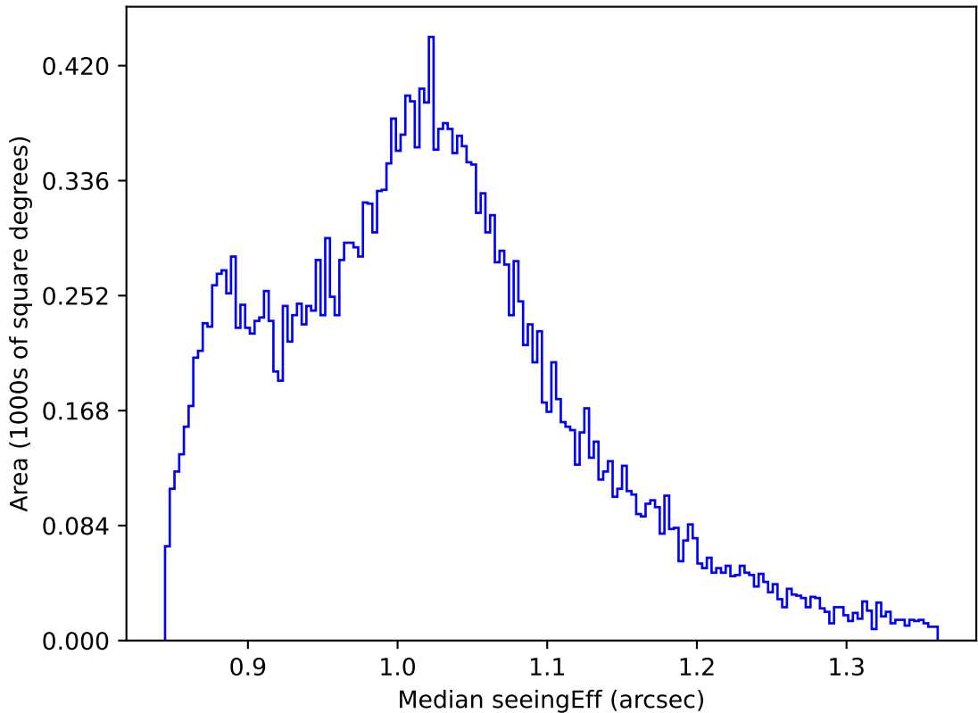
noroll_mjdp120_v3.4_10yrs All sky z band: Median seeingEff
