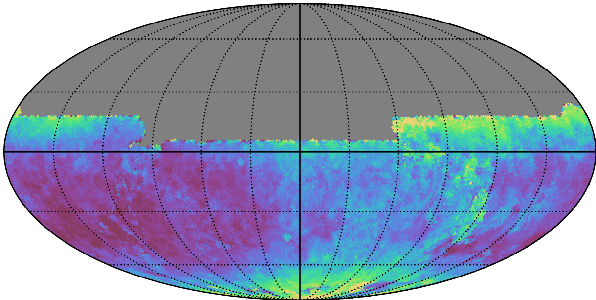
noroll_mjdp120_v3.4_10yrs All sky y band: Median seeingEff
